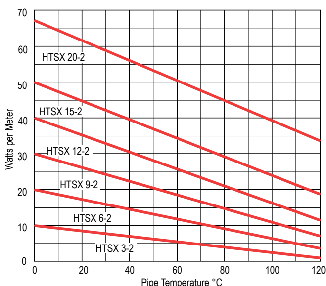
HTSX at 230 Vac
