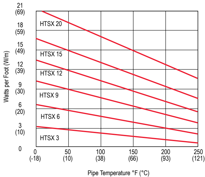
Graph 3.2 HTSX Power Output Curves at 120 Vac
