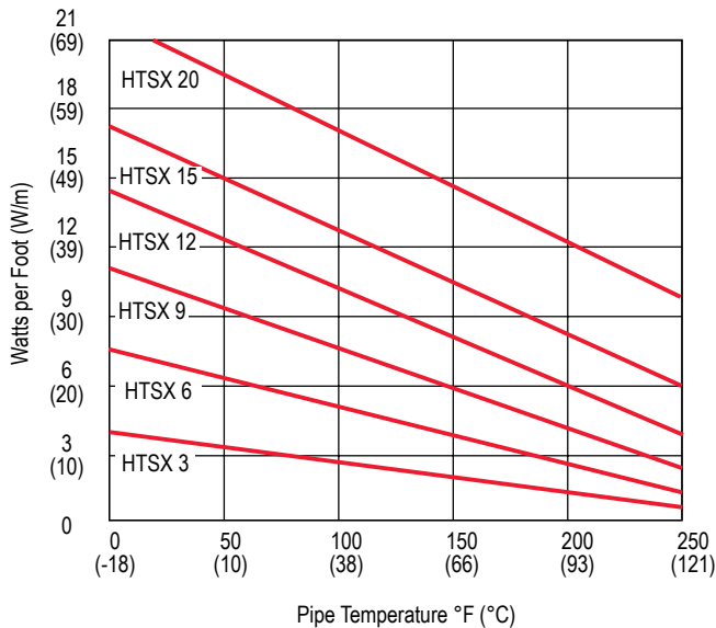
Graph 3.3 HTSX Power Output Curves at 240 Vac
