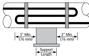
Pipe Support
